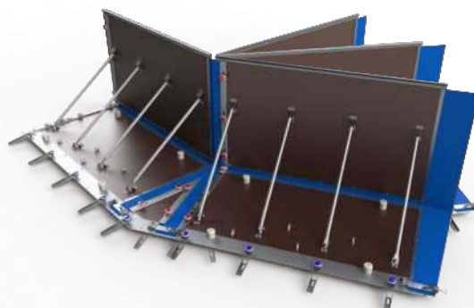
A variety of V1200 corner panels
