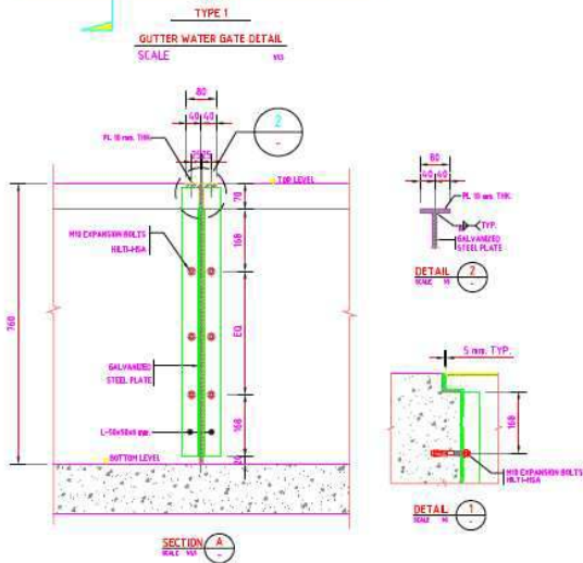
Drain Stop Glljotin
