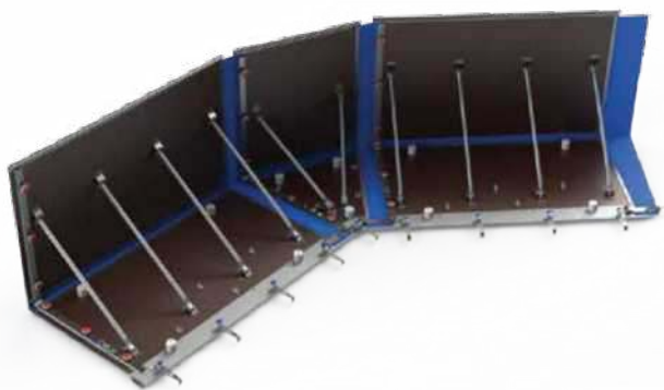
Inside 22.5 degree corner using v1200 panels
