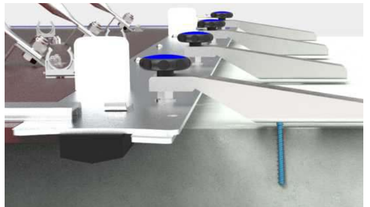
Tapcon Screws
